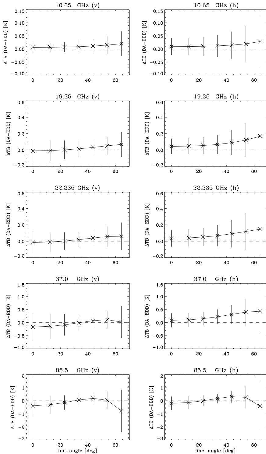
Figure 5: Mean DA-EDD differences at 10.65, 19.35, 22.235, 37.0, and 85.5 GHz (left panels: vertical polarization, right panels: horizontal polarization); error bars correspond to \pm one standard deviation.
