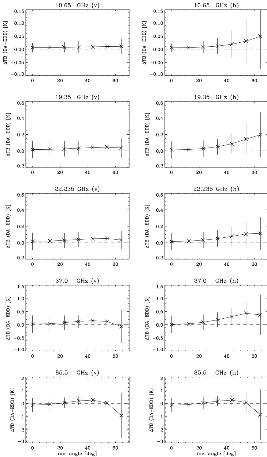
Figure 6: Same as Figure 5 for constant emissivities.
