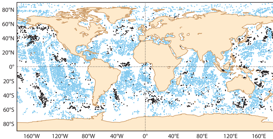
Figure 1 The distribution of overcast cloudy scenes (black dots) and completely clear scenes (blue dots) from the four infrared sensors MetOp-HIRS, NOAA-18 HIRS, MetOp-IASI and AQUA-AIRS during the first 12 hour analysis cycle from 00 UTC on 12 January 2008.
