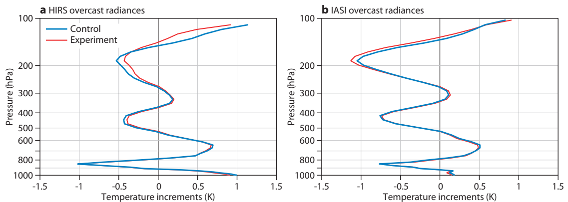
Figure 3 Vertical profiles of temperature increments from (a) HIRS overcast radiances with cloud altitudes diagnosed between 225 and 240 hPa and (b) IASI overcast radiances with cloud altitudes diagnosed between 195 and 215 hPa during the first 12-hour analysis cycle from 00 UTC on 12 October 2008 from two tropical locations east of Papua New Guinea.
