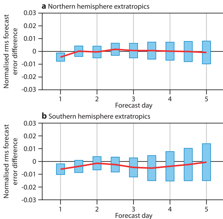
Figure 5 Normalized rms forecast error difference (experiment minus control divided by control) for 500 hPa geopotential height in (a) northern hemisphere extratropics (20°–90°N) and (b) southern hemisphere extratropics (20°–90°S) evaluated over 77 cases from the full test period. Each system is verified against its own analyses and the vertical error bars indicate 95% confidence intervals.
