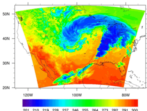
Simulated AIRS window channel
