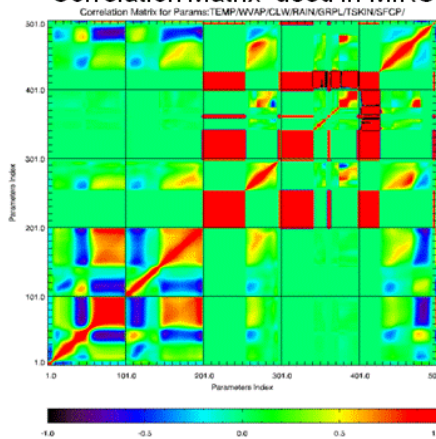
Correlation Matrix used in MiRS
