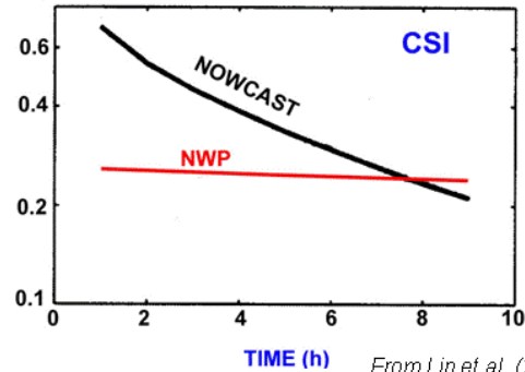
0.1 mm hourly precipitation skill scores over 21 days
