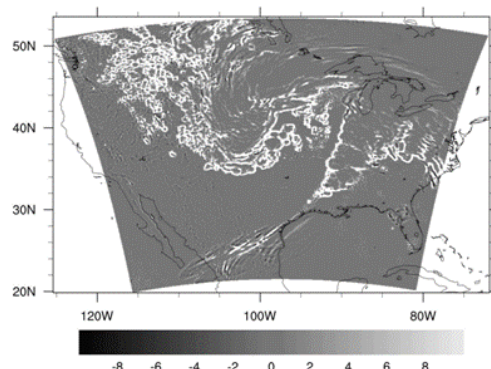
Simulated representativeness error
