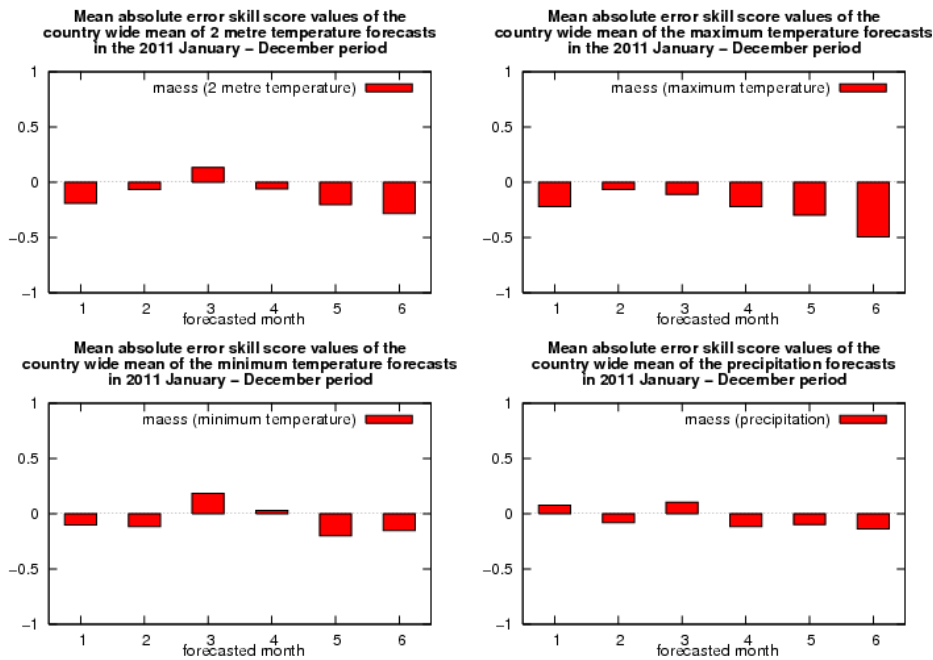
Figure 13 Mean Absolute Error Skill Score of ensemble means of 2 meter, maximum, minimum temperature and precipitation for the 6 forecasted months in a forecast for 2011. Reference forecast was the 30-year climatological mean.
