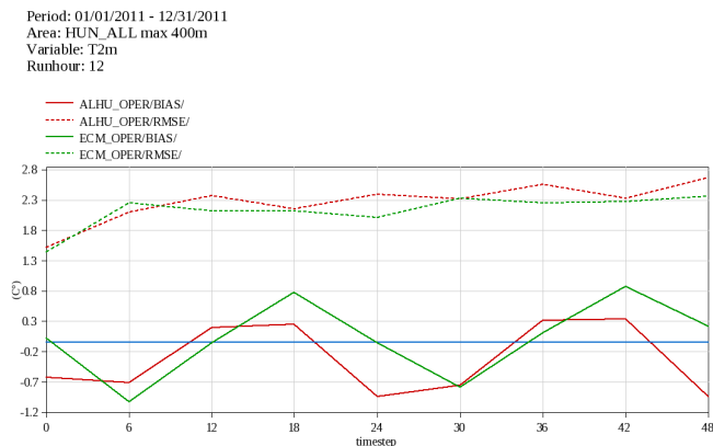
Figure 5 Comparison of BIAS and RMSE values for ECMWF (green) and ALADIN (red) 2m temperature forecasts over Hungary.
