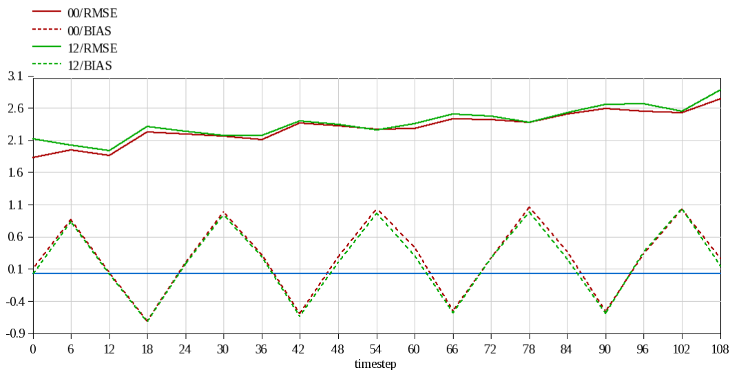
Figure 1 RMSE and BIAS values for ECMWF 2m temperature forecasts for Hungary. The RMSE values are slightly increasing with the forecast range and the BIAS fluctuates around zero with a strong diurnal cycle.
