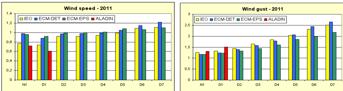
Figure 11 Mean Absolute Error (MAE) of wind speed and wind gust forecasts for different forecast ranges (D0 stands for the first night where relevant) in case of ALADIN (AL) , ECMWF Deterministic (EC Det) , ECMWF EPS mean (EC EPS) and the Operational Forecaster (Fo) for 2011 D0 represent the first night, D1, D2, ... etc the days after the issue of the forecast.
