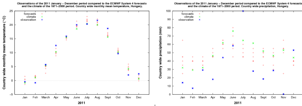
Figure 14 Comparison of the forecasts issued for the 2011 January-December period with the observations and the climate. Monthly mean temperature (left) and monthly amount of precipitation (right).
