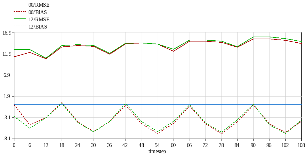
Figure 2 RMSE and BIAS values for ECMWF 2m relative humidity forecasts for Hungary. The RMSE values are slightly increasing with the forecast range and the BIAS fluctuates with a strong diurnal cycle.
