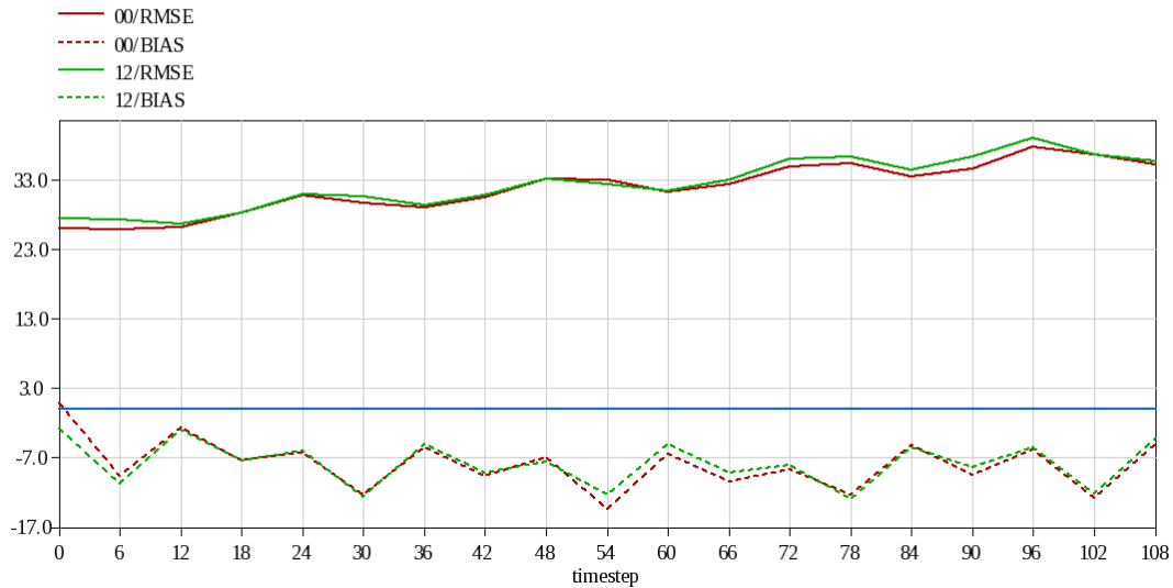
Figure 4 RMSE and BIAS values for ECMWF total cloudiness forecasts for Hungary. There is a cloudiness underestimation at all ranges (around -5 and -10 percent).
