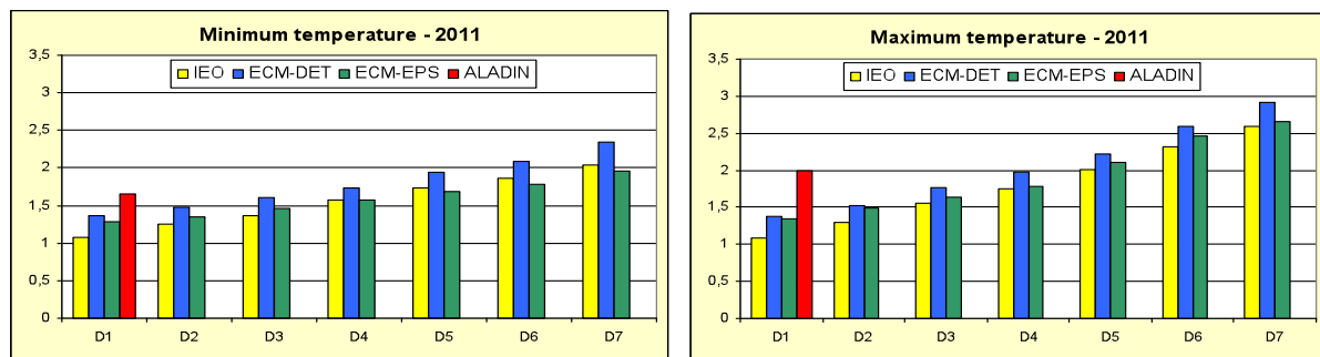
Figure 9 Mean Absolute Error (MAE) of minimum, maximum and daily mean temperature for different forecast ranges (D0 stands for the first night where relevant) in case of ALADIN (AL), ECMWF Deterministic (EC Det), ECMWF EPS mean (EC EPS) and the Operational Forecaster (Fo) for 2011 D0 represent the first night, D1, D2, ... etc the days after the issue of the forecast.
