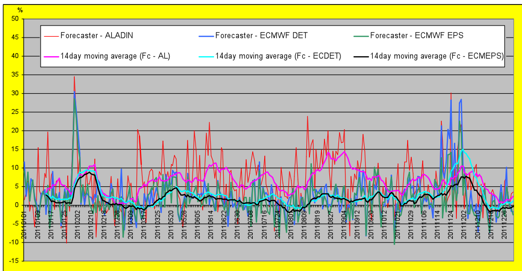
Figure 12 Difference of the daily Complex Score for the first day calculated for the Forecaster and the models in 2011 (difference between the Forecaster and ALADIN , the Forecaster and ECMWF DET as well as Forecaster and EXMWF EPS mean ). 14 day moving averages are also shown.
