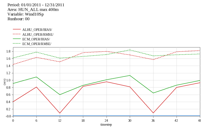
Figure 7 Comparison of BIAS and RMSE values for ECMWF (green) and ALADIN (red) wind speed forecasts over Hungary. In RMSE there is no significant difference between the two model forecasts, in BIAS ALADIN is better than ECMWF.
