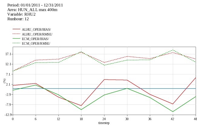
Figure 6 Comparison of BIAS and RMSE values for ECMWF (green) and ALADIN (red) 2m relative humidity forecasts over Hungary.
