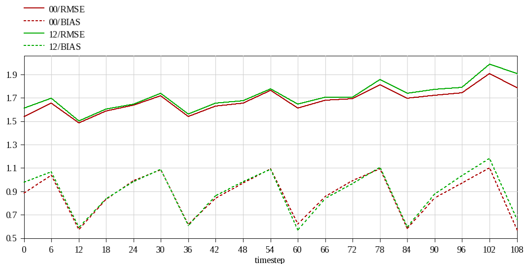
Figure 3 RMSE and BIAS values for ECMWF 10m wind speed forecasts for Hungary. The RMSE values are rather constant in the first couple days, then there is a slight increase afterwards. The BIAS fluctuates in a diurnal cycle at a range of about 0.3 m/s (first 3 days) and about 0.5m/s (later).
