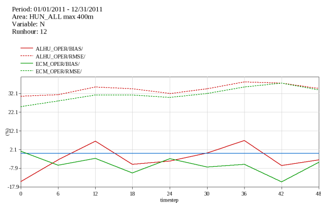
Figure 8 Comparison of BIAS and RMSE values for ECMWF (green) and ALADIN (red) total cloudiness forecasts over Hungary. RMSE values of the ECMWF forecasts are smaller than that of the ALADIN ones during all time ranges. There is a systematic underestimation in the ECMWF forecasts.
