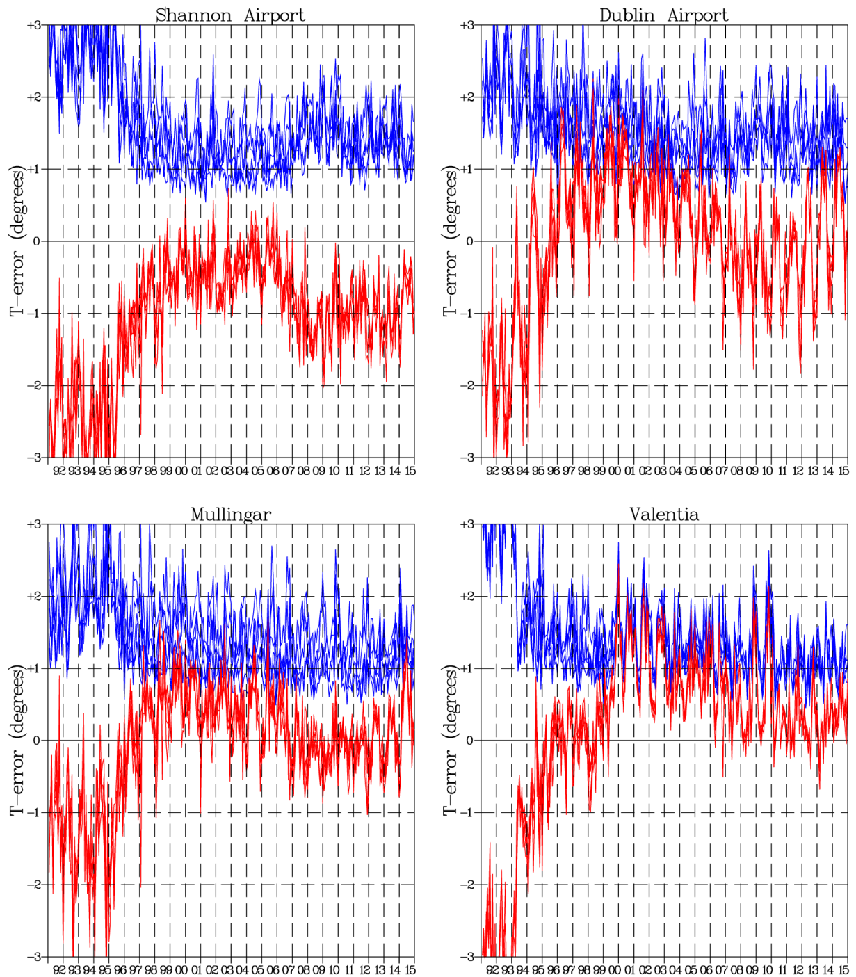
Figure 2 Scores for the T+12, T+36, T+60, T+84, and T+108 ECMWF forecasts of 2-metre Temperature. Note that all these forecasts verify at midnight. The blue lines show values of the monthly mean of the absolute error, the red lines values of the monthly mean of the mean error or bias.
