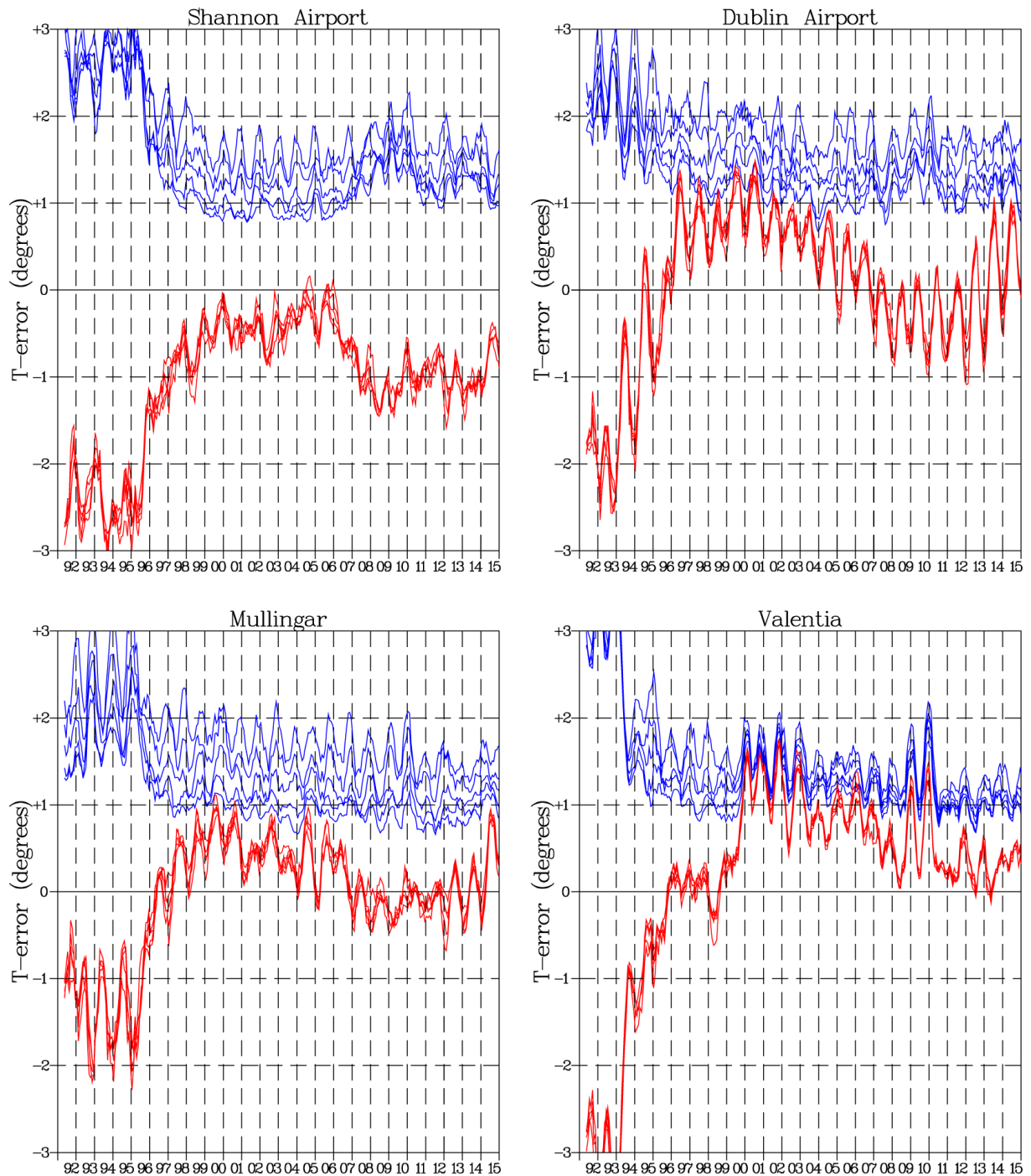
Figure 4 Smoothed scores for the T+12, T+36, T+60, T+84, and T+108 ECMWF forecasts of 2-metre Temperature verifying at midnight. The lines were smoothed by taking a 5-month centred running mean. The blue lines show values of the monthly mean of the absolute error, the red lines values of the monthly mean of the mean error or bias. The top blue line corresponds to a T+106 forecast, the one below that to a T+84 forecast etc.
