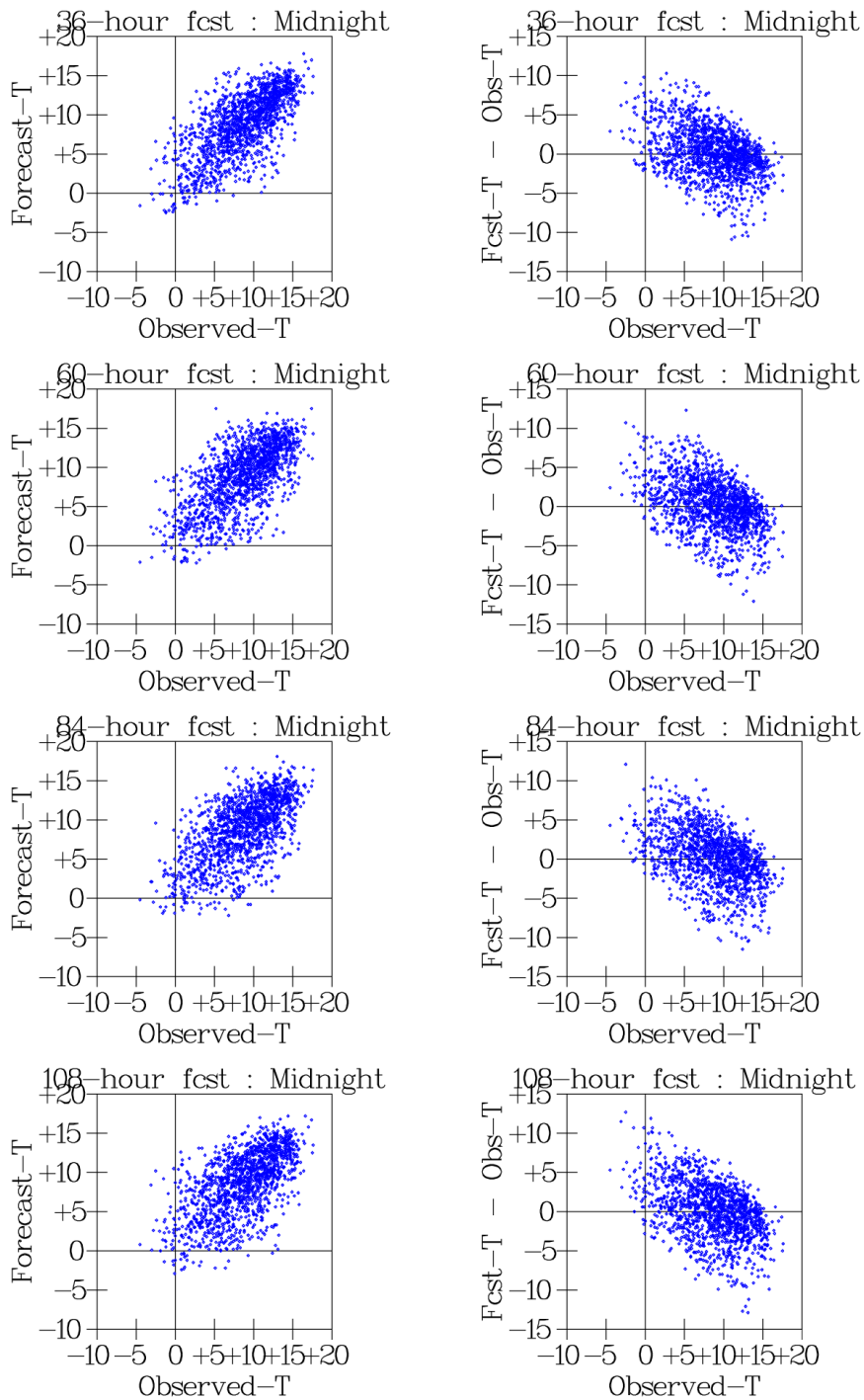
Figure 9 Scatter plots for ECMWF forecasts of 2-metre Temperature, in 2015. All forecasts verify at midnight and the four stations have been combined.
