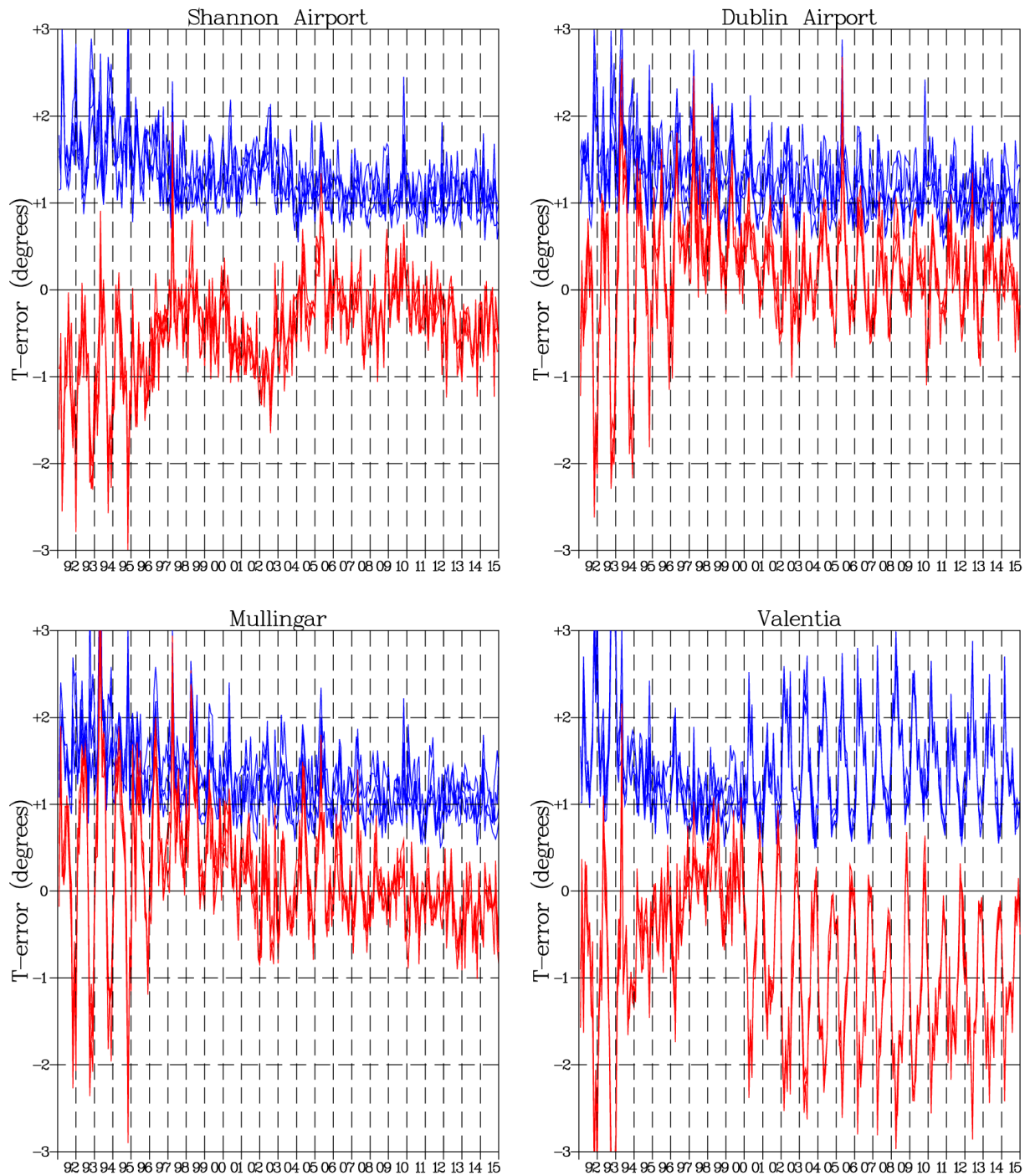
Figure 1 Scores for the T+24, T+48, T+72, and T+96 ECMWF forecasts of 2-metre Temperature. Note that all these forecasts verify at midday. The blue lines show values of the monthly mean of the absolute error, the red lines values of the monthly mean of the mean error or bias.
