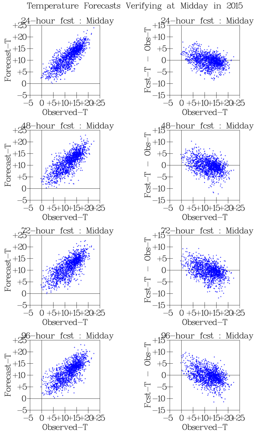
Figure 8 Scatter plots for ECMWF forecasts of 2-metre Temperature, in 2015. All forecasts verify at midday and the four stations have been combined.
