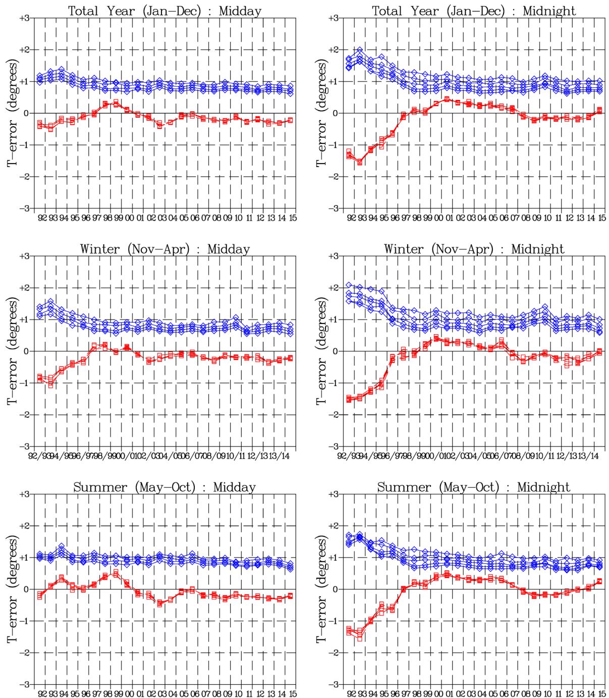
Figure 6 Mean seasonal and yearly scores for ECMWF forecasts of 2-metre Temperature averaged over four stations. The blue lines indicate the error [mean absolute error], the red lines the bias [mean error]. Note that in 1992 the bias was much larger for the forecasts verifying at midnight rather than at midday but this effect became much less in later years [red lines]. Similarly, the error was greater, in 1992, for the midnight runs but gradually, over time, the difference became less [blue lines]. The errors for the various forecast lengths can be distinguished from the graphs: in all cases the top blue line corresponds to the longest forecast, the bottom blue line to the shortest.
