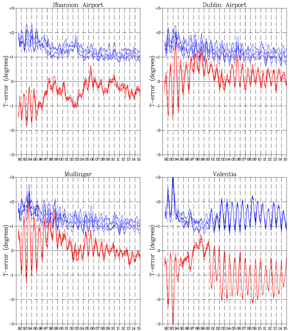
Figure 3 Smoothed scores for the T+24, T+48, T+72, and T+96 ECMWF forecasts of 2-metre Temperature verifying at midday. The lines were smoothed by taking a 5-month centred running mean. The blue lines show values of the monthly mean of the absolute error, the red lines values of the monthly mean of the mean error or bias. The top blue line corresponds to a T+96 forecast, the one below that to a T+72 forecast etc.
