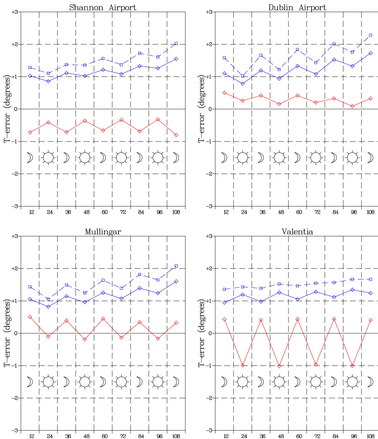
Figure 7 Mean scores for ECMWF forecasts of 2-metre Temperature, in 2015, averaged over a year of data. The solid blue line is the mean absolute error, the dashed blue line the rms error and the red line the mean error or bias. It can be seen that the quality of the forecast decreases with the length of the forecast. The 'sun' and 'moon' symbols indicate forecasts verifying at midday and midnight, respectively. The length of the forecast [in hours] is indicated on the x-axis.
