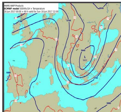
500hPa GH-T for 18-06-2017 12UTC
