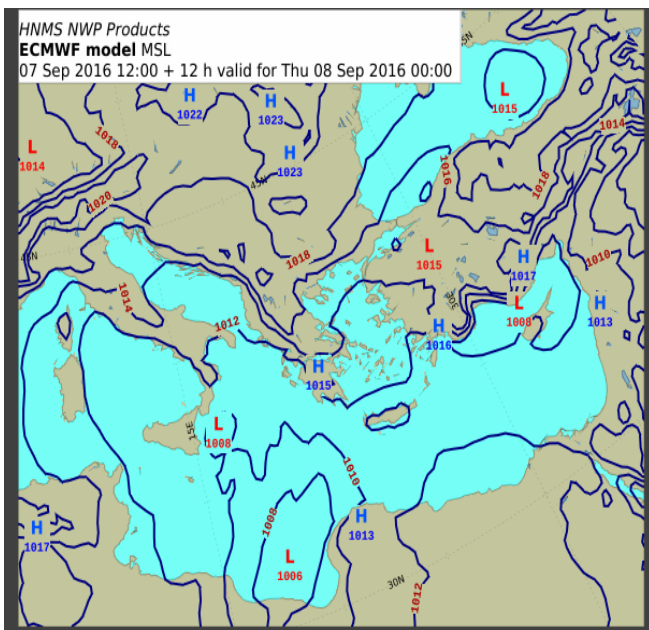
MSLP for 08-09-2016 00UTC
