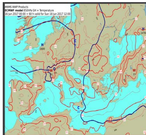
850hPa GH-T for 18-06-2017 12UTC
