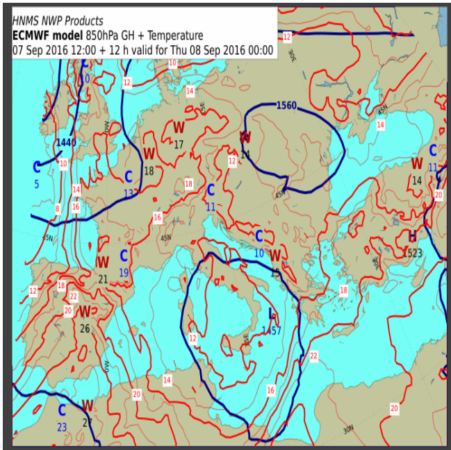
850hPa GH-T for 08-09-2016 00UTC
