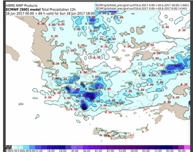
12HR TOTAL PRECIPITATION FORECAST FROM ECMWF FOR 18-06-2017 18UTC
