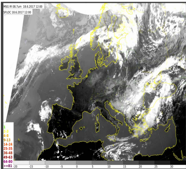
MSG IR IMAGE FOR 18-06-2017 12UTC
