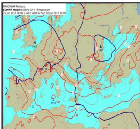
850hPa GH-T for 18-06-2017 00UTC
