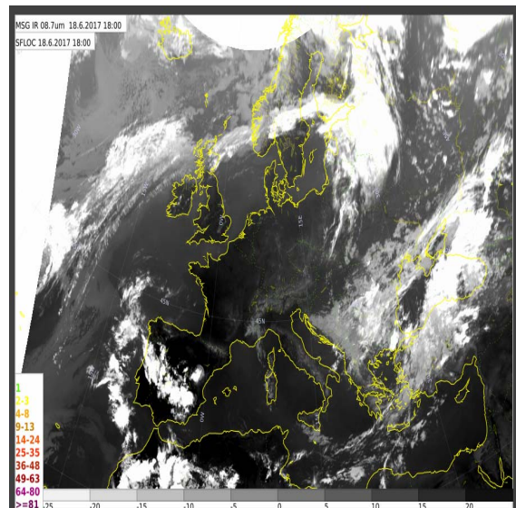
MSG IR IMAGE FOR 18-06-2017 18UTC
