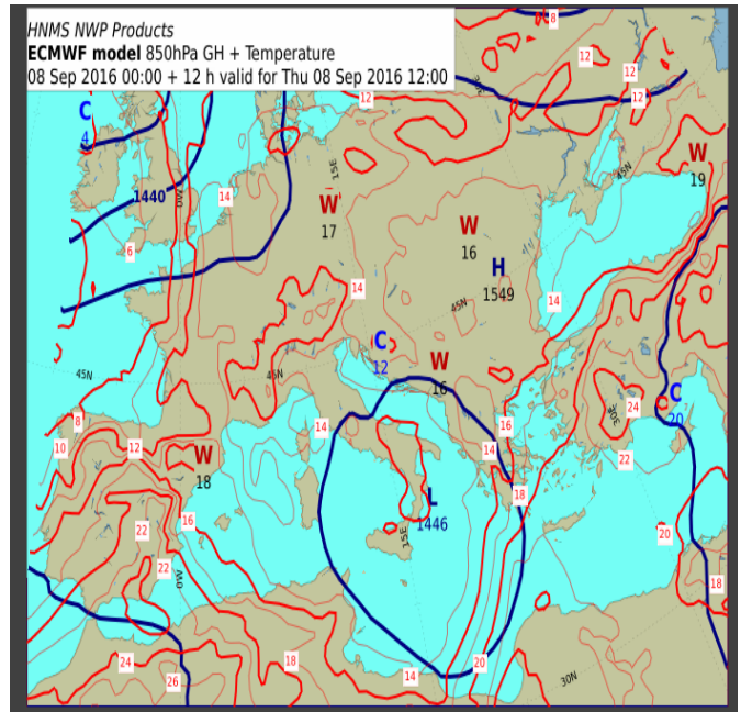
850hPa GH-T for 08-09-2016 12UTC
