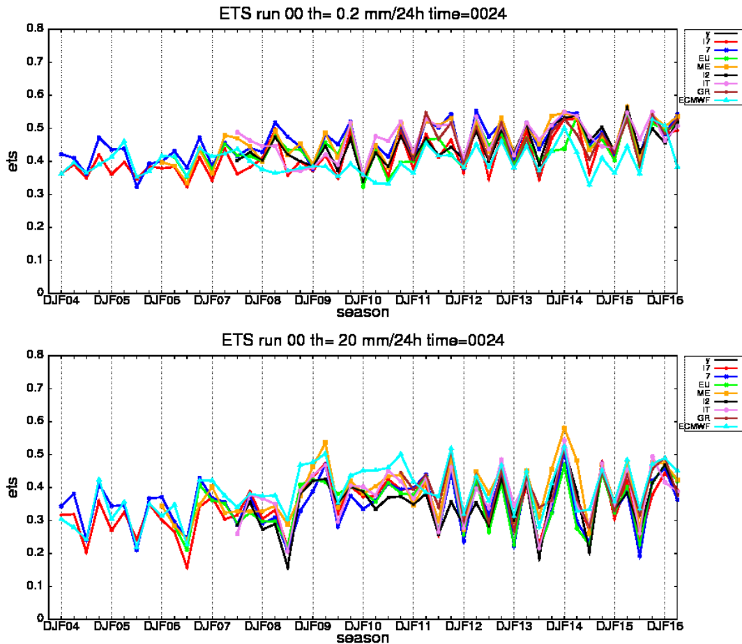
Fig.6: Long-term trend of ETS for various COSMO implementations in comparison with IFS for two thresholds 0.2mm/24h and 20mm/24h.
