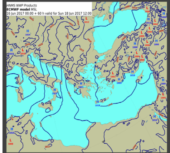
MSLP for 18-06-2017 12UTC
