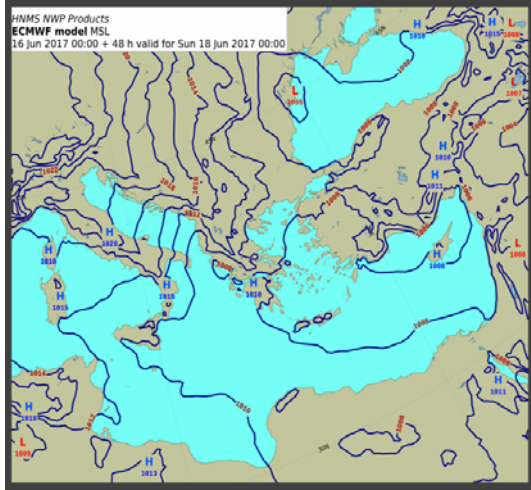
MSLP for 18-06-2017 00UTC
