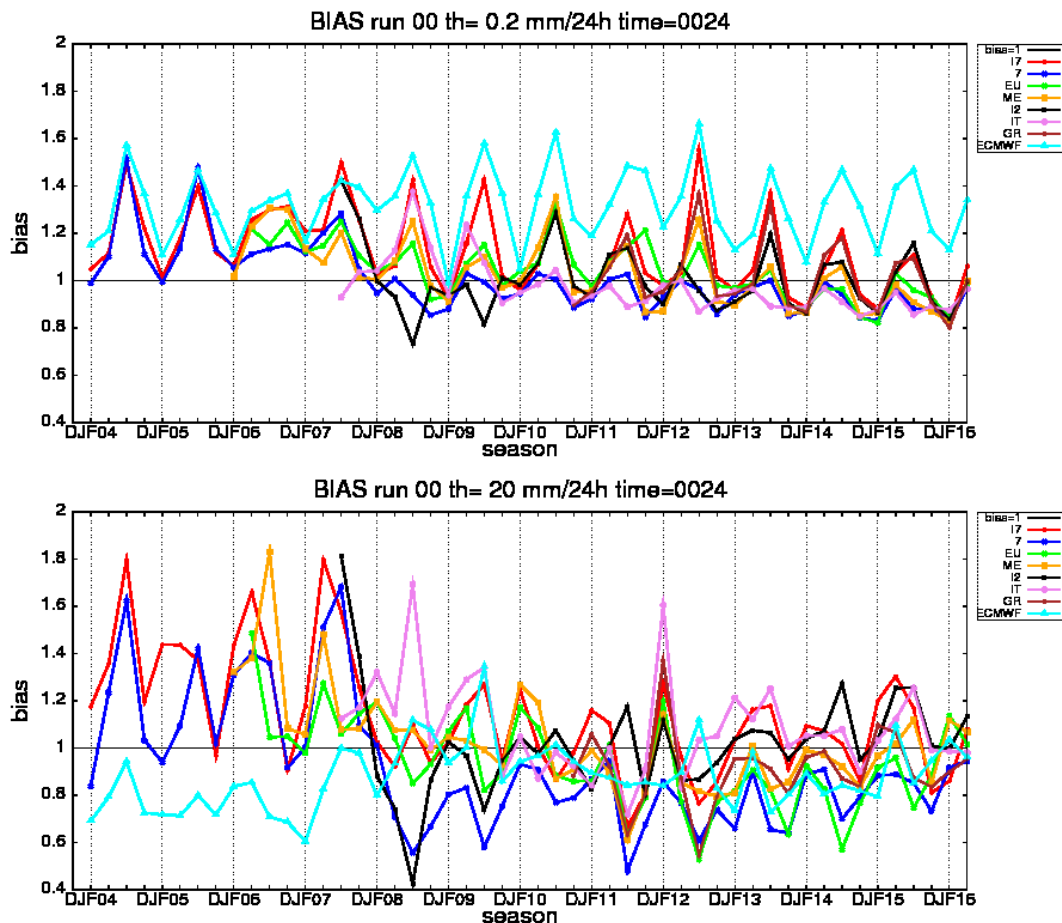
Fig.5: Long-term trend of BIAS for various COSMO implementations in comparison with IFS for two thresholds 0.2mm/24h and 20mm/24h.
