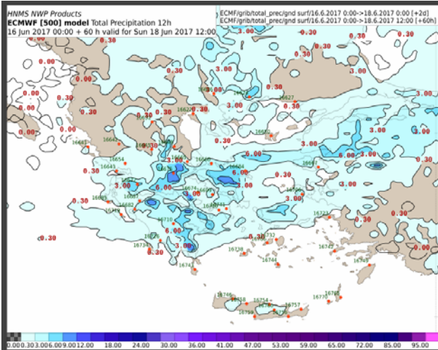
12HR TOTAL PRECIPITATION FORECAST FROM ECMWF FOR 18-06-2017 12UTC
