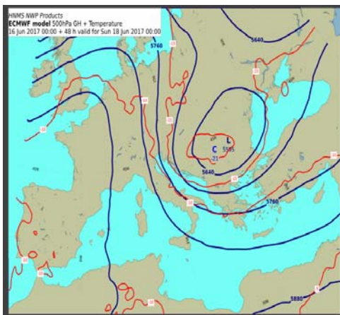
500hPa GH-T for 18-06-2017 00UTC
