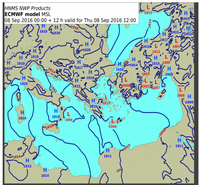
MSLP for 08-09-2016 12UTC
