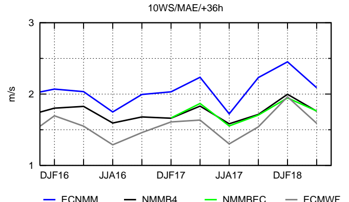
Fig.15-16 ME and MAE of ECMWF midday (36h) 10 meter wind speed forecast for seasons DJF16 to MAM18. Comparison to operational NWP models forecast.
