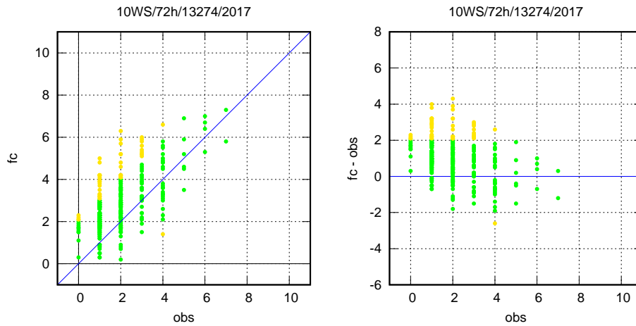
Fig.4 Scatterplot and forecast errors vs. observations of one year ECMWF t+72h (midnight) 10 meter wind speed forecast for Beograd - Karadordev park (13274).
