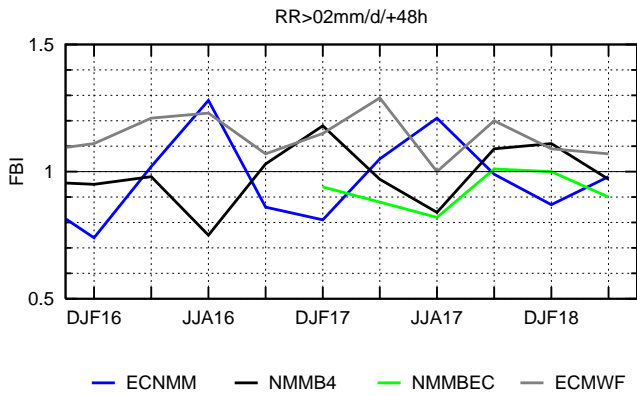
Fig.17-18 FBI and ETS of ECMWF 24h precipitation forecast (48h) for seasons DJF16 to MAM18. Threshold is 2mm/24h. Comparison to operational NWP models forecast
