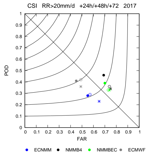
Fig.19-20 CSI contours as a function of FAR and POD for 24h/48h/72h 24h precipitation forecast Thresholds are 2mm/24h and 20mm/24h. Comparison to operational NWP models forecast
