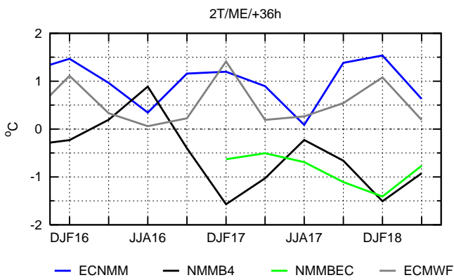
Fig.13-14 ME and MAE of ECMWF midday (36h) 2 meter temperature forecast for seasons DJF16 to MAM18. Comparison to operational NWP models forecast.
