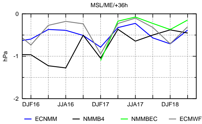
Fig.11-12 ME and MAE of ECMWF midday (36h) mean sea level pressure forecast for seasons DJF16 to MAM18. Comparison to operational NWP models forecast.
