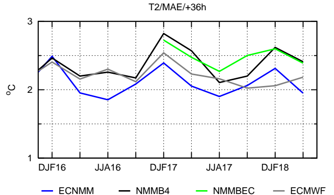
Fig.13-14 ME and MAE of ECMWF midday (36h) 2 meter temperature forecast for seasons DJF16 to MAM18. Comparison to operational NWP models forecast.
