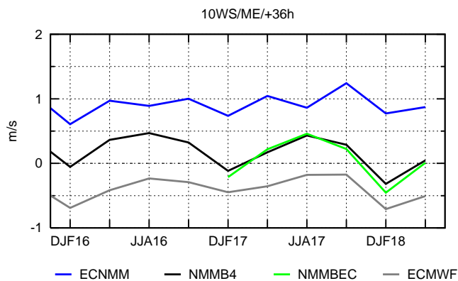
Fig.15-16 ME and MAE of ECMWF midday (36h) 10 meter wind speed forecast for seasons DJF16 to MAM18. Comparison to operational NWP models forecast.
