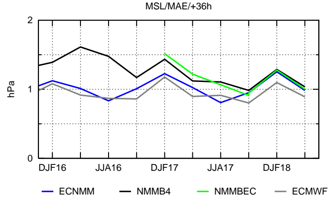
Fig.11-12 ME and MAE of ECMWF midday (36h) mean sea level pressure forecast for seasons DJF16 to MAM18. Comparison to operational NWP models forecast.
