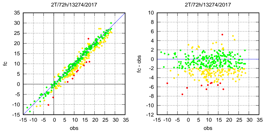
Fig.3 Scatterplot and forecast errors vs. observations of one year ECMWF t+72h (midnight) 2 meter temperature forecast for Beograd - Karađorđev park (13274).
