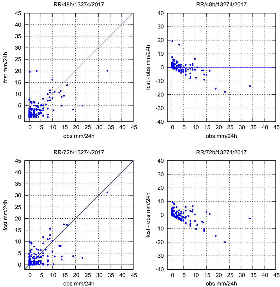
Fig.9-10 Scatterplots and forecast errors vs. observations of one year ECMWF 48h and 72h 24h precipitation forecast for Beograd - Karadorđev park (13274).
