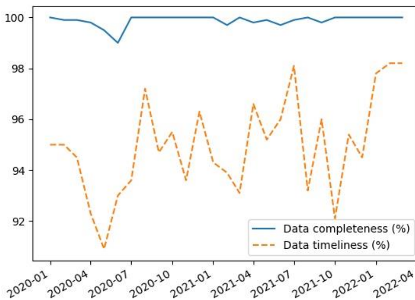
Figure 2: Monthly SMOS NN nominal soil moisture production completeness and delivery timeliness percentages (see text for how these are calculated) for the period January 2020 to March 2022
