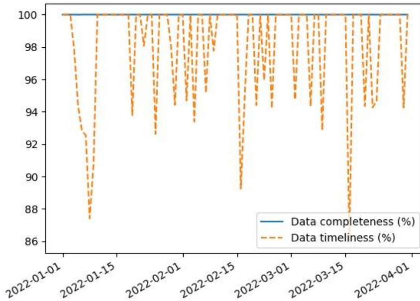
Figure 1: Daily SMOS NN nominal soil moisture production completeness and delivery timeliness percentages (see text for how these are calculated) for the first quarter of 2022: 1 st January to 31 st March 2022
