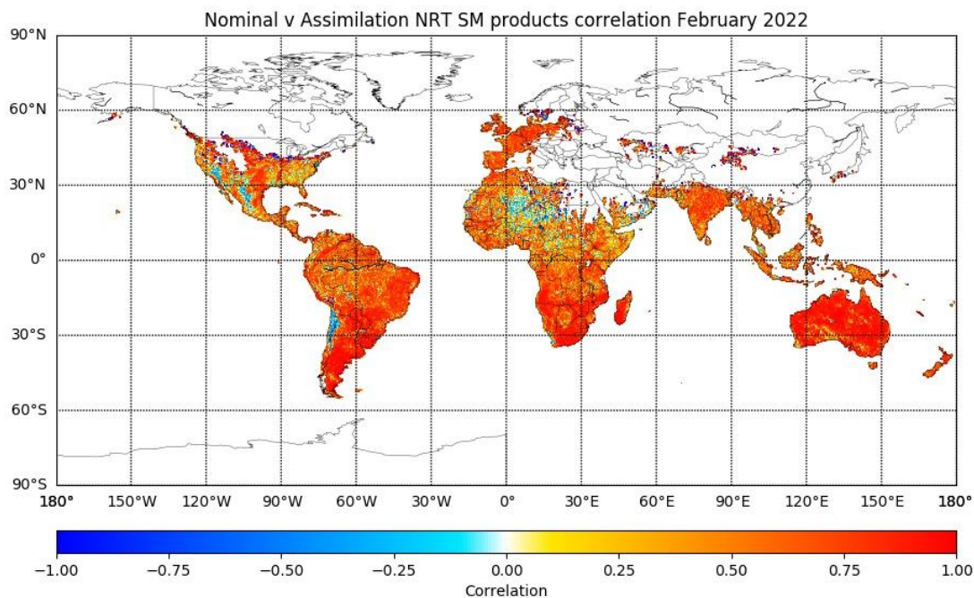
Figure 4: Correlation between the ESA nominal neural network product and the ECMWF assimilation neural network product in February 2022
