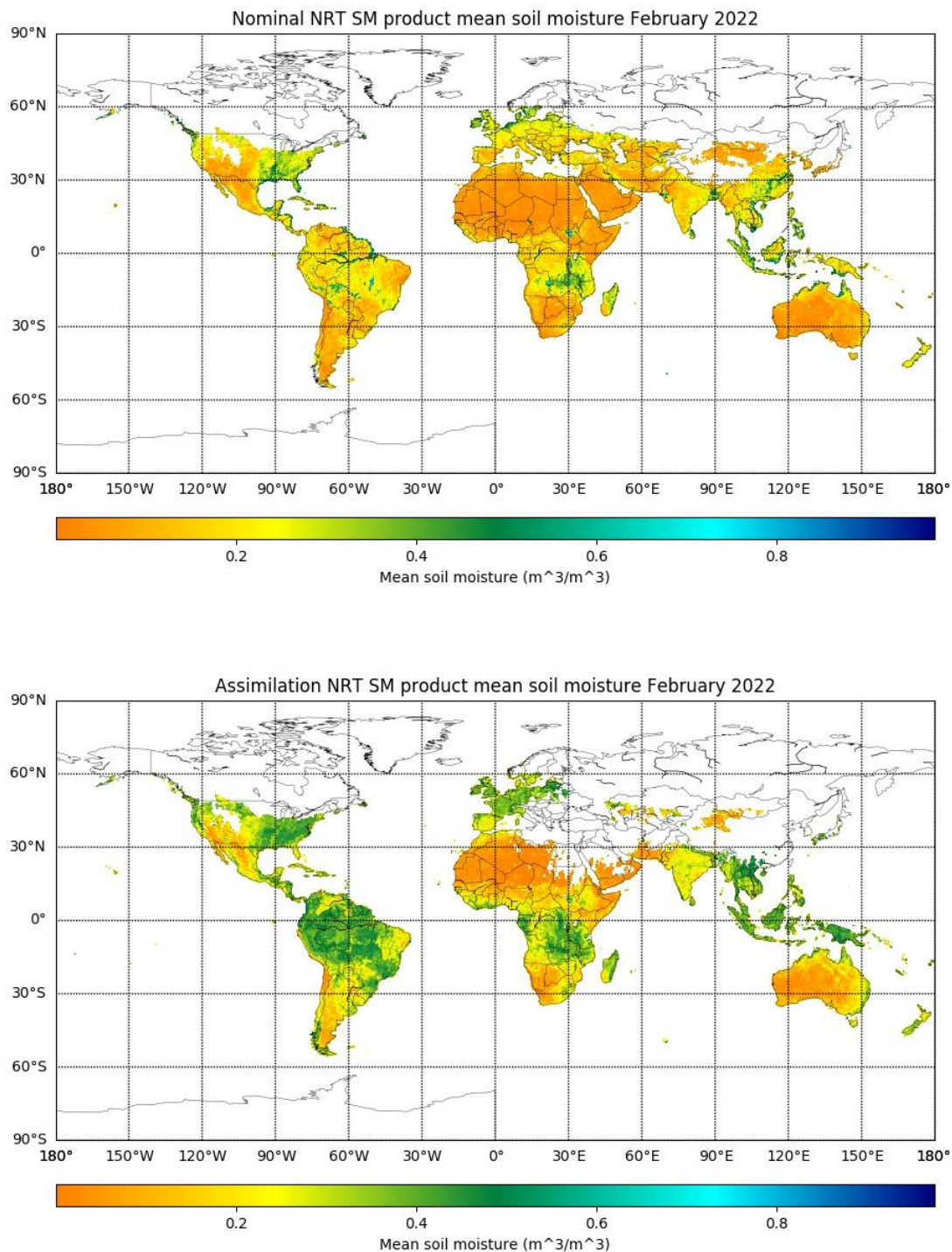
Figure 3: Mean retrieved soil moisture (m 3 /m 3 ) for February 2022 for the nominal NRT product (upper) and assimilation NRT product (lower)
