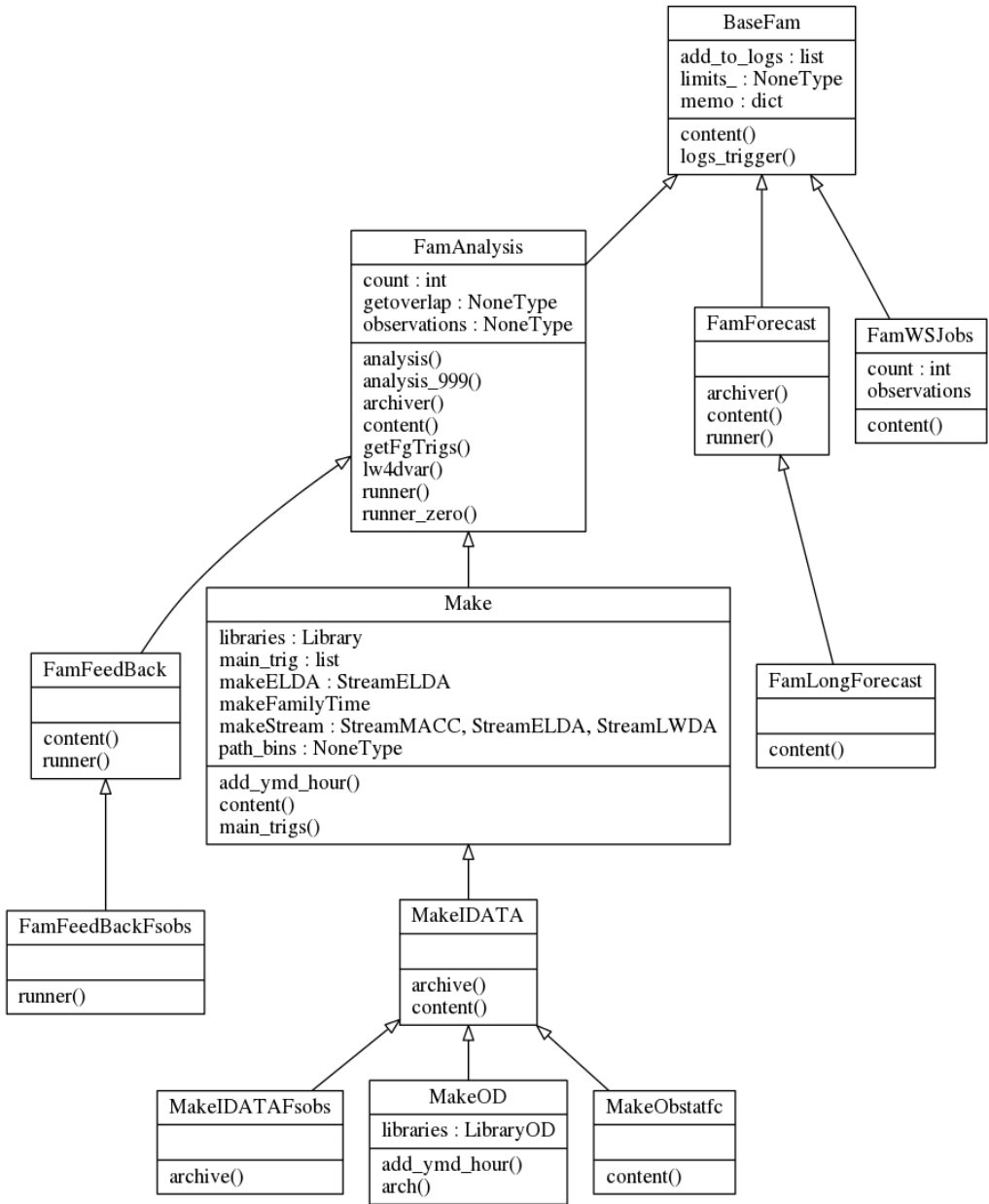
Class Diagram for module inc_fam.py.
