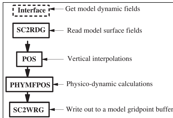
Figure 2.13 Vertical interpolations and physico-dynamic calculations on input grid: VPOS.
