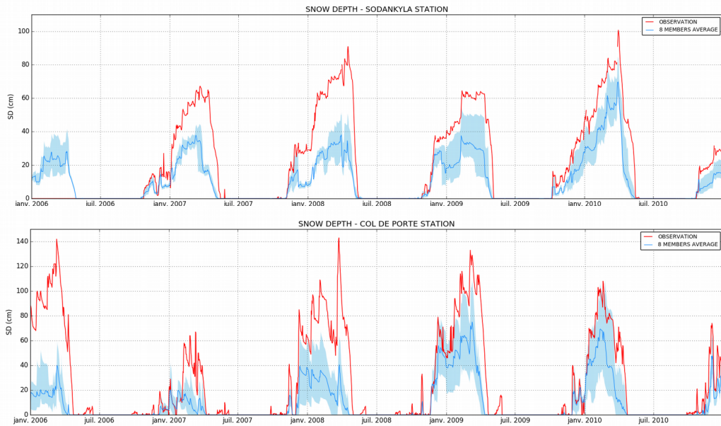
Fig 18: Sodankyla (Top) and Col de Porte (Alps) snow depth. Red: observations not used in the MESCAN-SURFEX-ENS. Blue area: defined by the extreme value of the 8 members. Blue line: mean of the ensemble.
